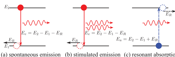
Figure 28. The influence of recoil on stimulated emission and resonant absorption. E_1 and E_2 are the level energies. The resonant gamma-ray energy for spontaneous and stimulated emission E_e is lower than E_2 - E_1 by the recoil energy E_R , while the gamma-ray energy required for resonant absorption E_a is higher than the internal energy difference, again, by the recoil energy. Thus, the emitted photons are detuned from resonance and are not readily absorbed.
