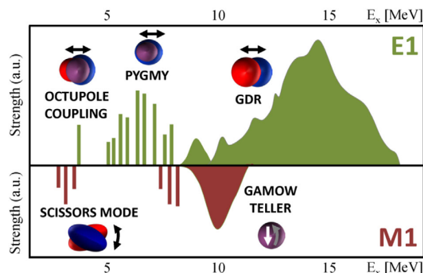
Figure 7. Illustration of the photoresponse of deformed atomic nuclei as a function of the photon energy, divided into phenomena involving electric (E1) and magnetic (M1) excitations. Figure by A. Zilges.
