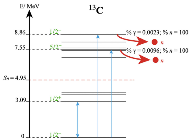
Figure 8. Nuclear energy levels below 8.86 MeV in ^{13}\text{C} . Energies, J^\pi and decay modes [55] are given for the levels discussed in this work. The arrows show excitation to be induced by the secondary GF photons. For the lowest-energy gamma resonance, the double-sided arrow indicates that the only decay channel is via photon emission.
