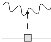
Figure 5. The \pi^0 -pole contribution to the PVTV polarizabilities. The square denotes the PVTV pion–nucleon coupling \tilde{g}_0 .
