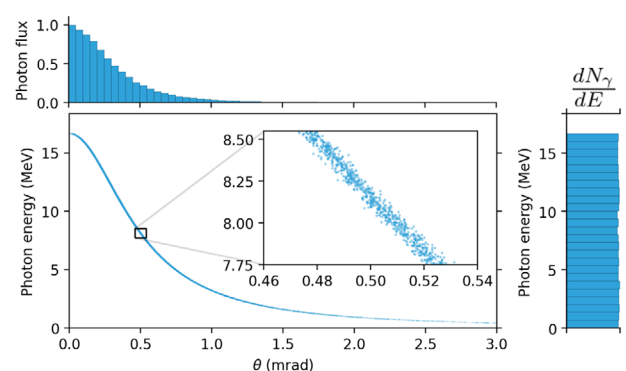
Figure 2. Correlation between the energy and angle of emitted photon in one particular case of the Gamma Factory based on hydrogen-like calcium ion beam in the LHC. The top histogram shows the corresponding photon flux density (photons per unit area per unit time) into a small solid angle. The right histogram shows the flat energy spectrum. The ion beam parameters in this example are: \gamma = 2048 , \sigma_x = 0.44 mm, \sigma_{x'} = 2.2 \mu\text{rad} (normalized emittance \epsilon_n = \gamma\sigma_x\sigma_{x'} = 2 mm-mrad). [11]
